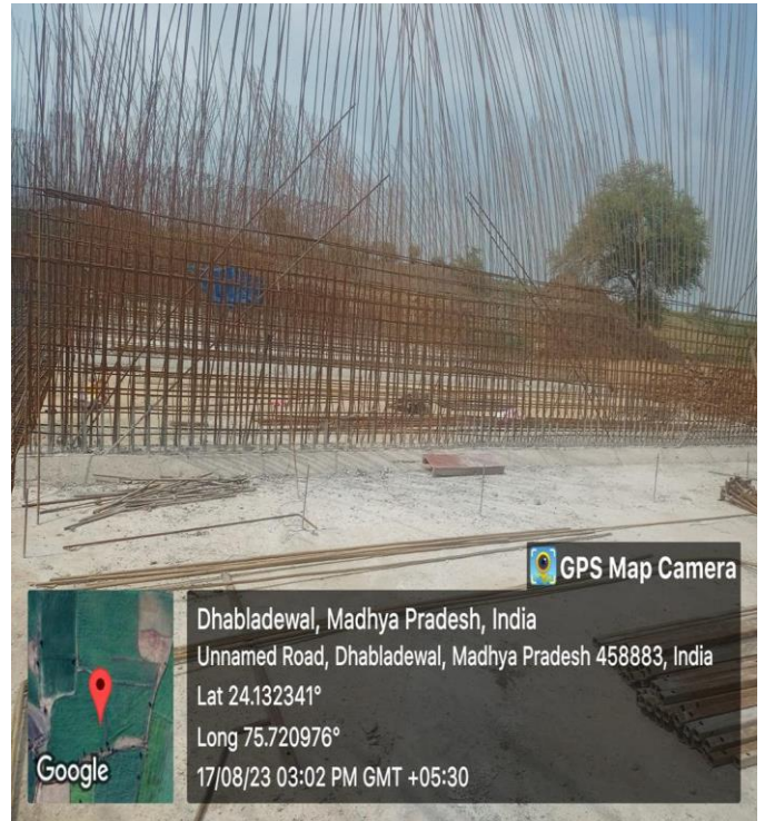
MJB Raft Completed at Ch- 113+817
