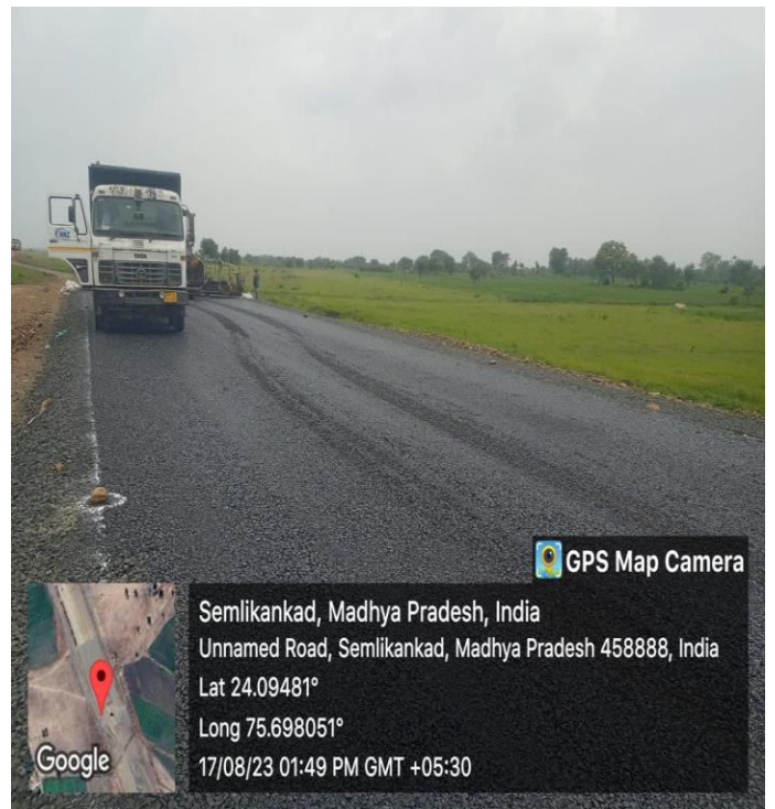
Prime coat WIP at Ch 112+409 LHS
